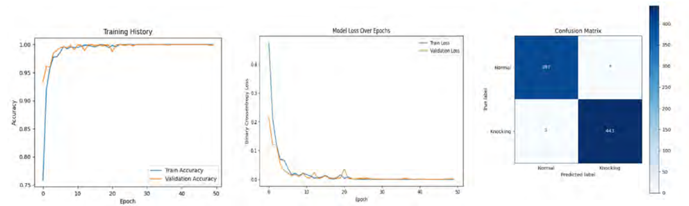
Knocking Detection: Accuracy, Loss curves and Confusion matrix
