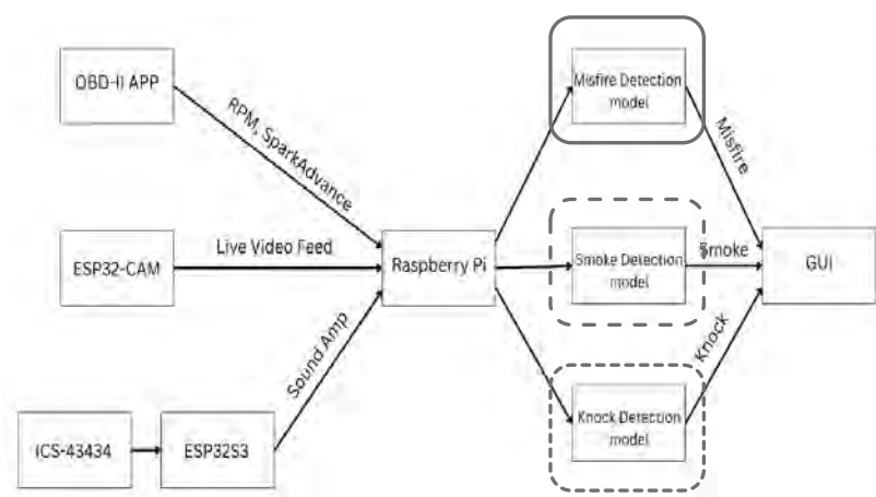
System Architecture of Engine Health monitoring system
